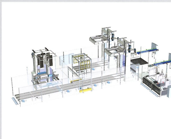
Transfer multiplo rulli e cinghie 5 vie
